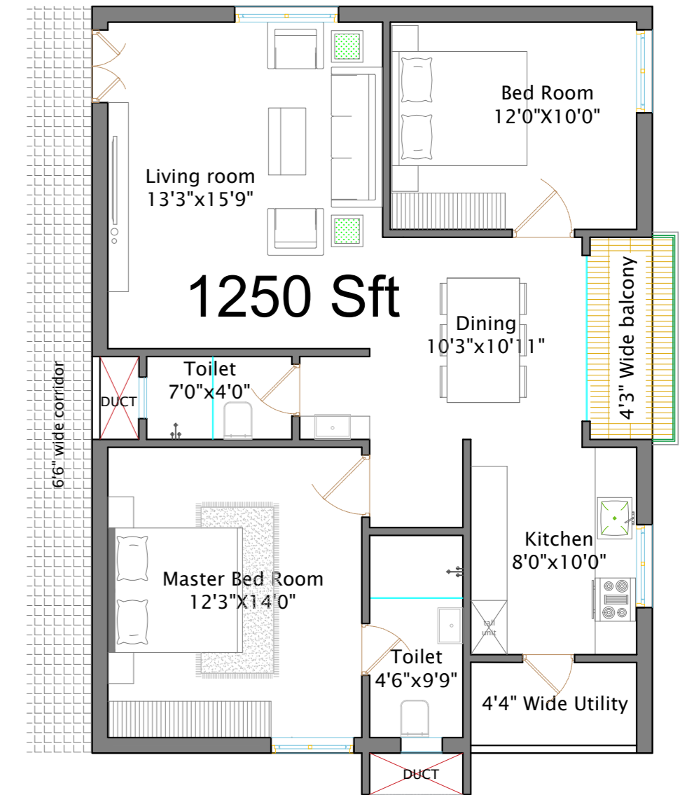
1250 Sft WEST FACING
