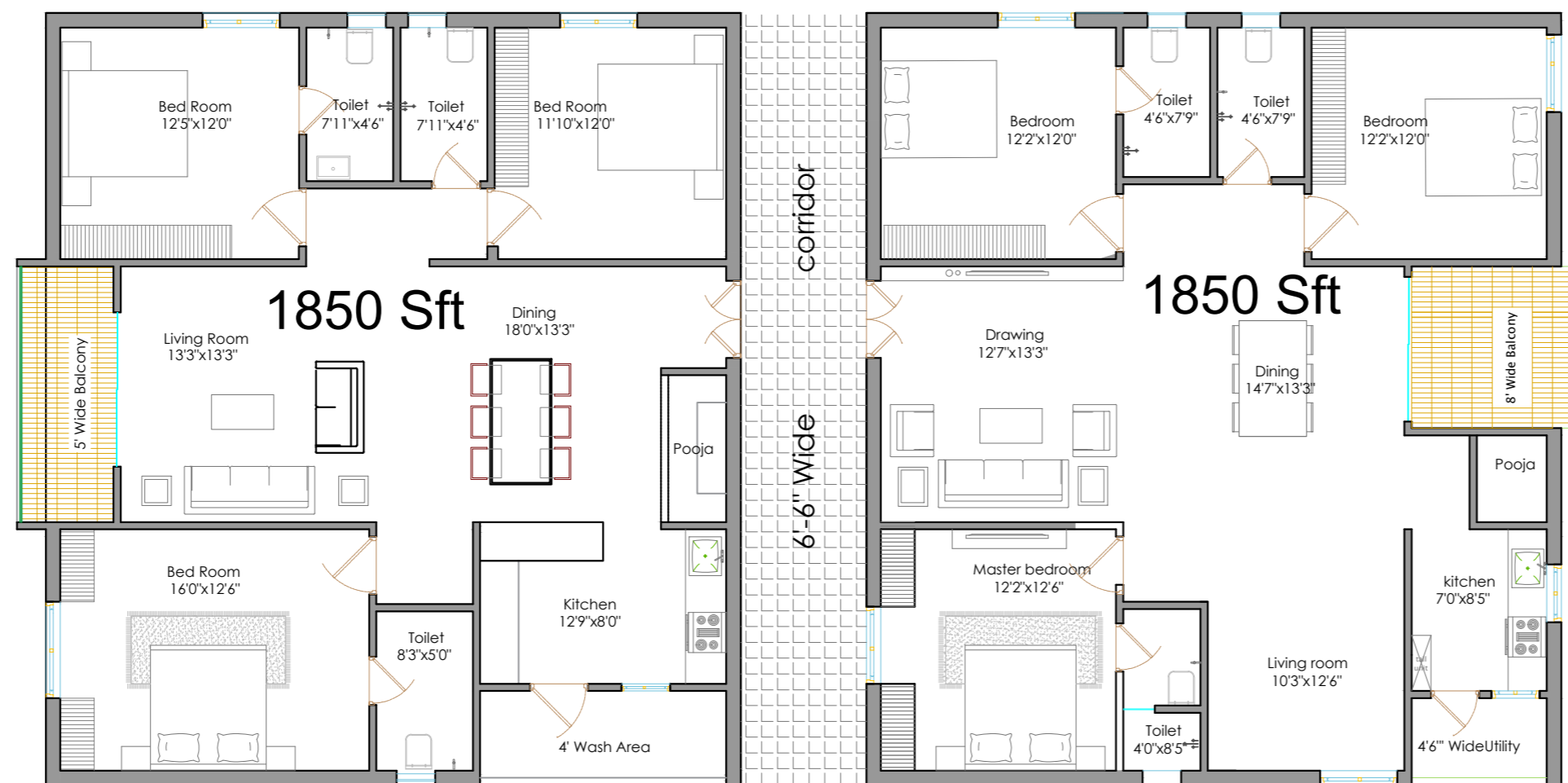
1850 Sft EAST FACING
