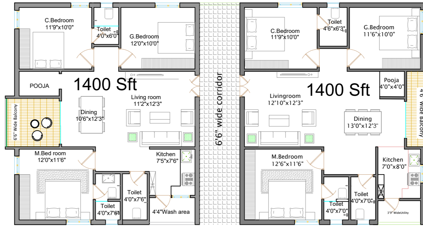
1400 Sft EAST FACING
