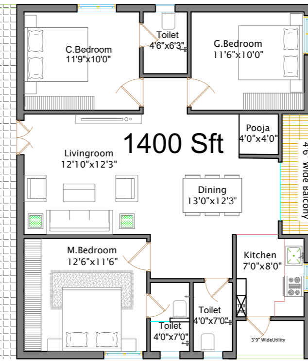
1400 Sft EAST FACING
